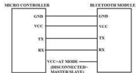
Fig-5: Typical application circuit
